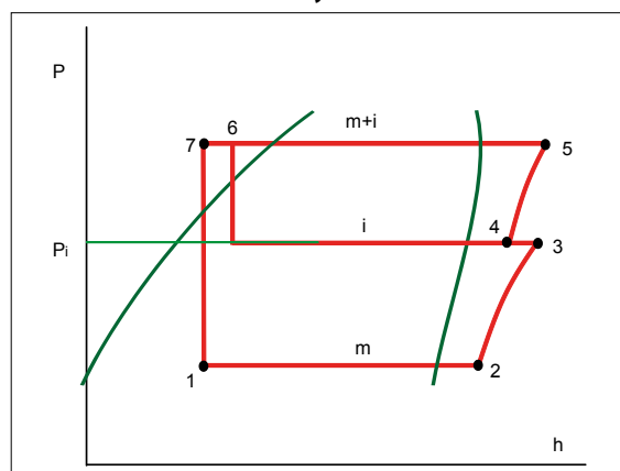
Economizer cycle 12345671
